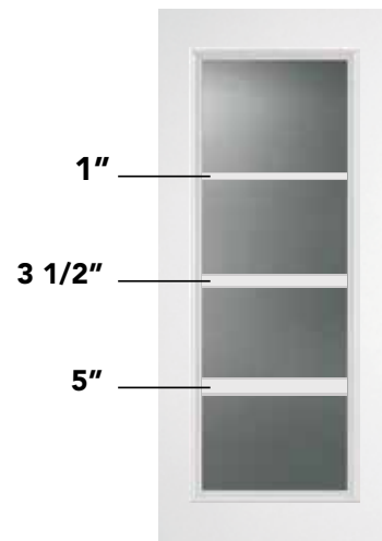
Full Horizontal 4 Lite 6/8 & 8/0 DRS00(80)-SDLFH436 SLS00(80)-SDLFH436
